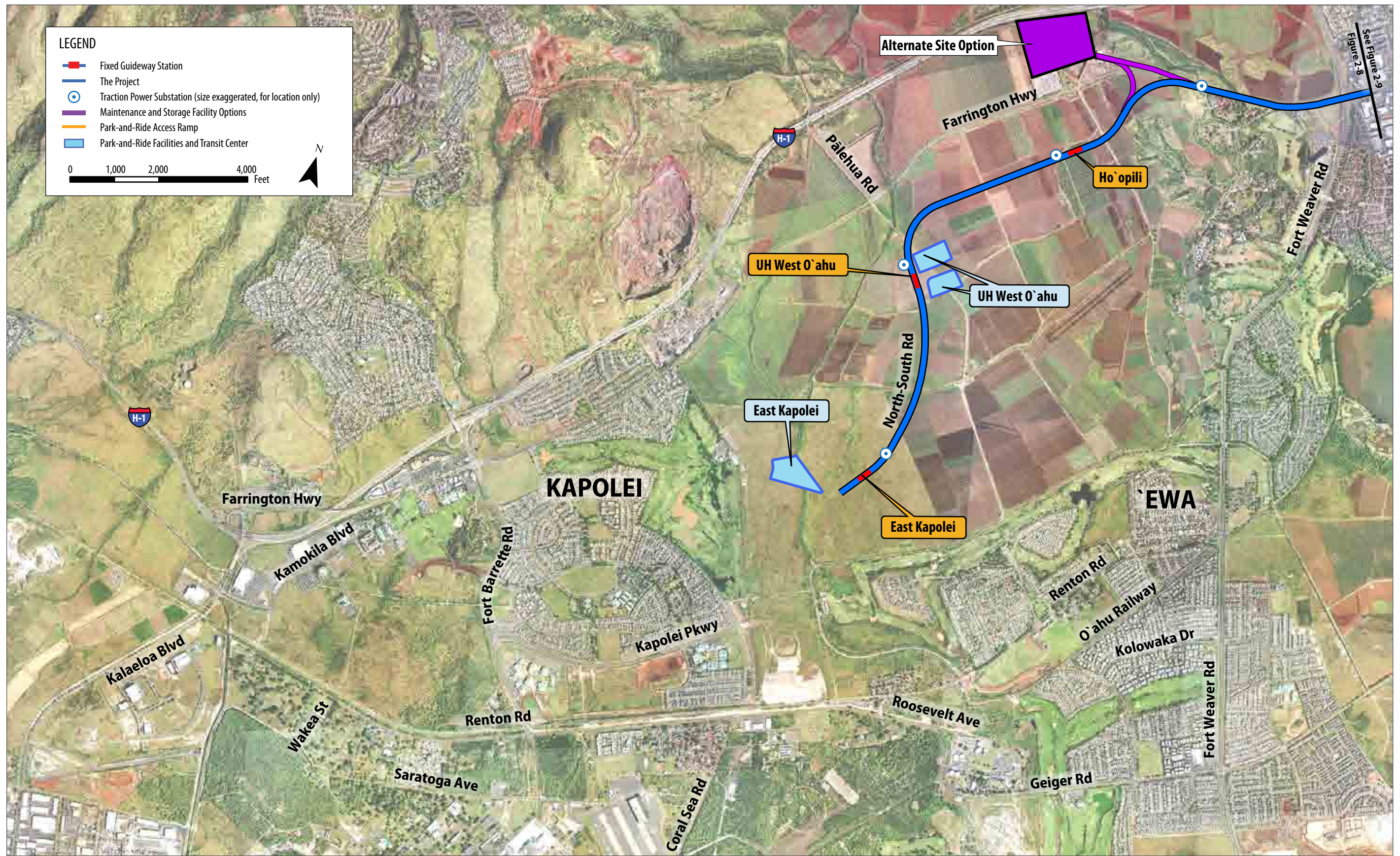
Figure 2-8 Fixed Guideway Transit Alternative Features (East Kapolei to Fort Weaver Road)
