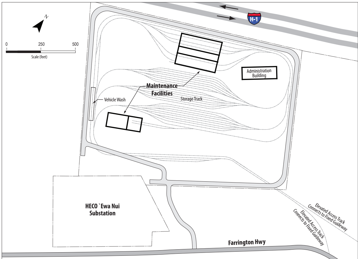
Figure 2-39 Maintenance and Storage Facility in Ho'opili Location and Conceptual Layout
