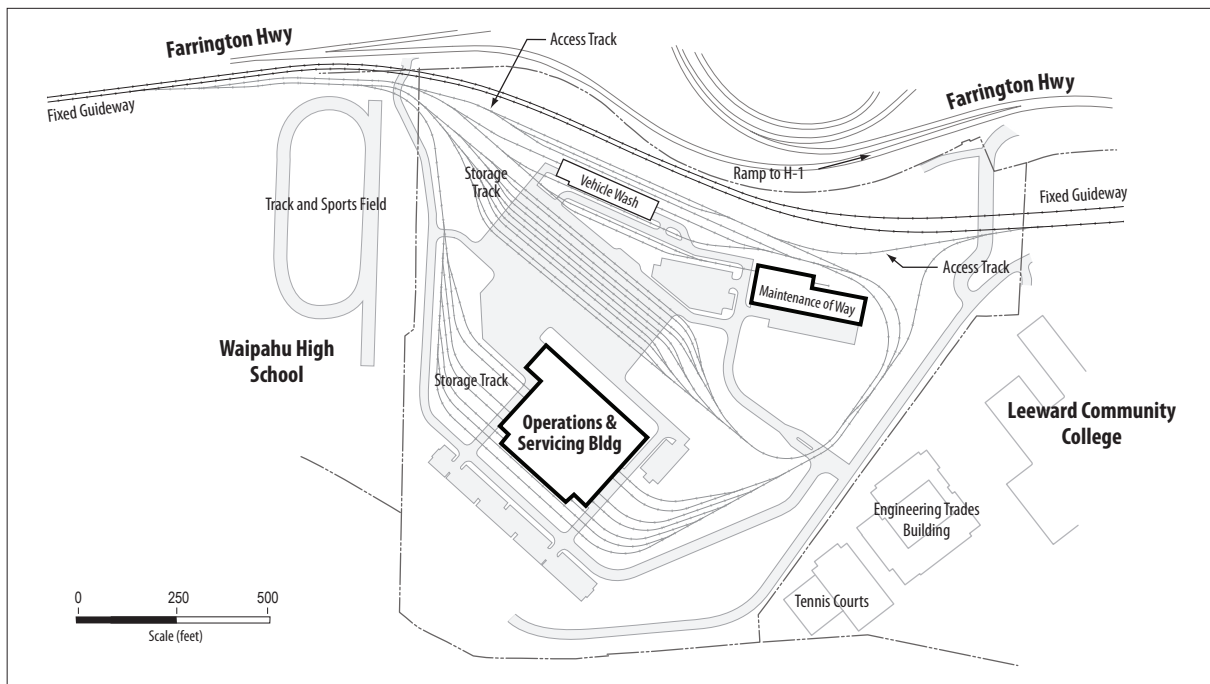
Figure 2-38 Leeward Community College Maintenance and Storage Facility Location and Conceptual Layout
