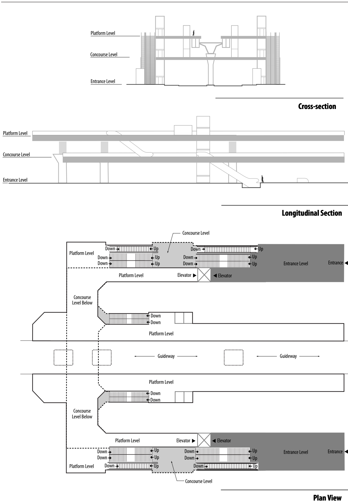
Figure 2-14 Typical Side-platform Station Configuration with a Concourse
