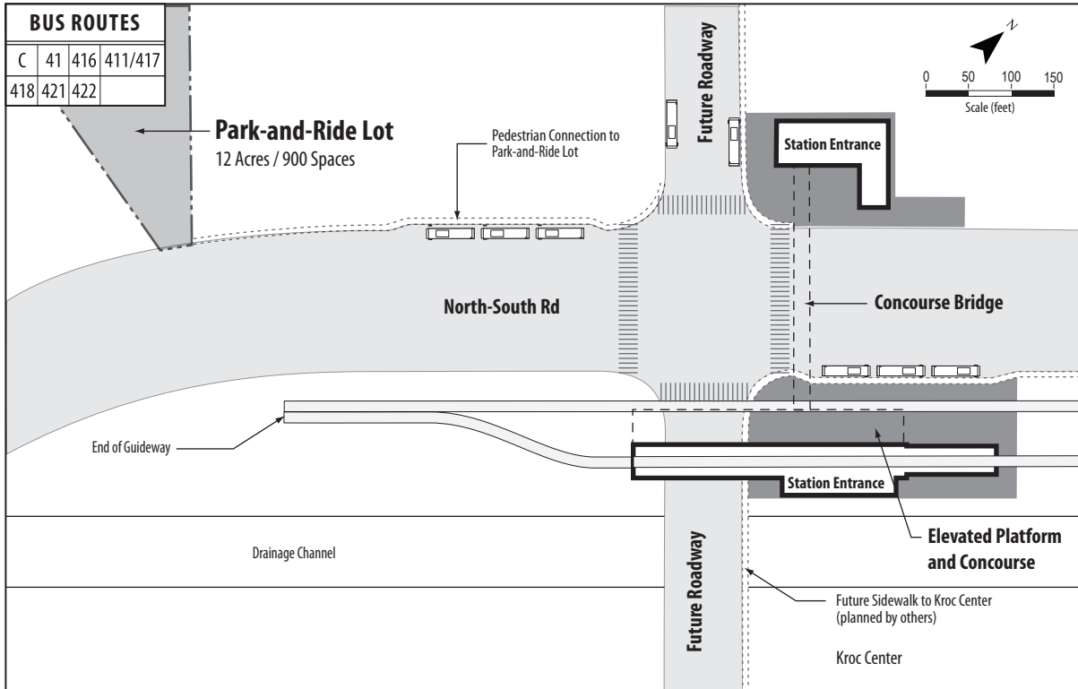
Figure 2-17 East Kapolei Station
