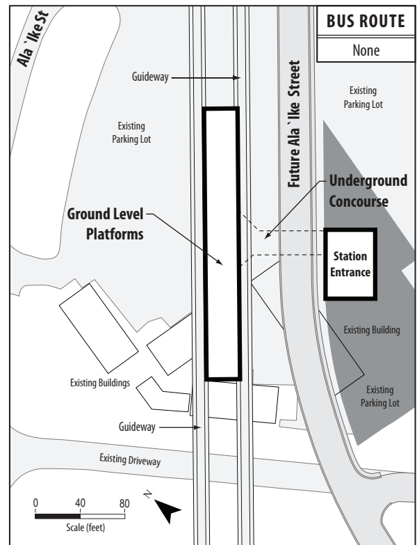
Figure 2-22 Leeward Community College Station
