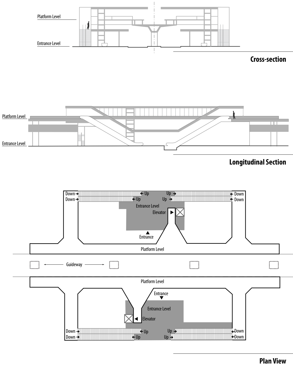
Figure 2-13 Typical Side-platform Station Configuration without a Concourse
