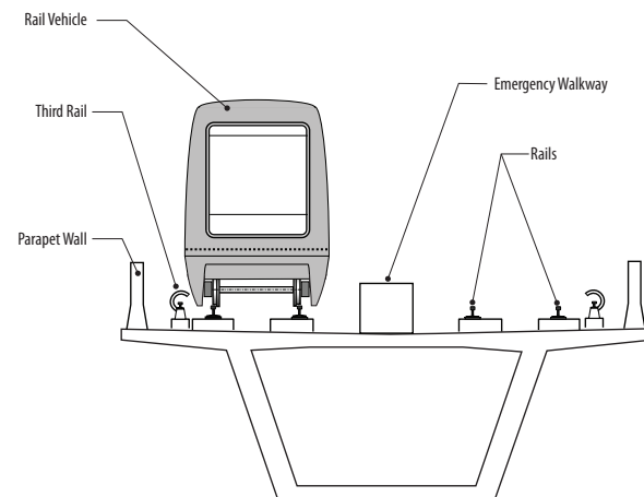
Figure 2-12 Example Vehicle on Elevated Guideway (Cross-section)
