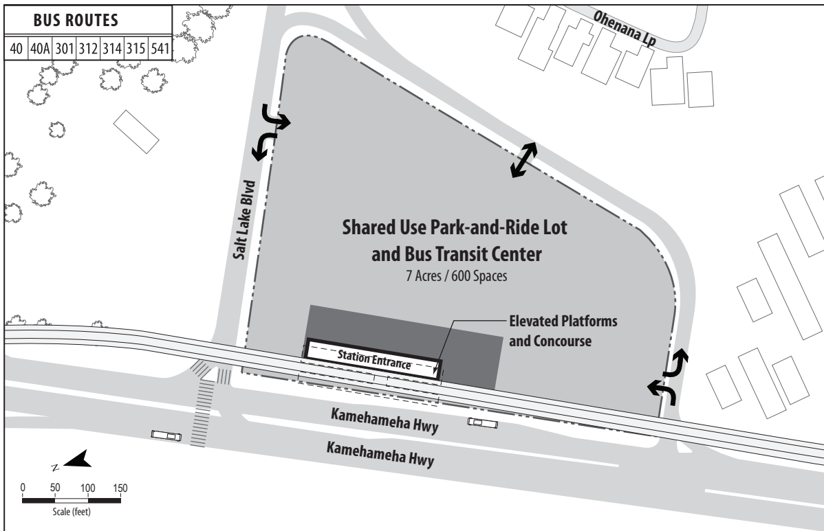
Figure 2-25 Aloha Stadium Station
