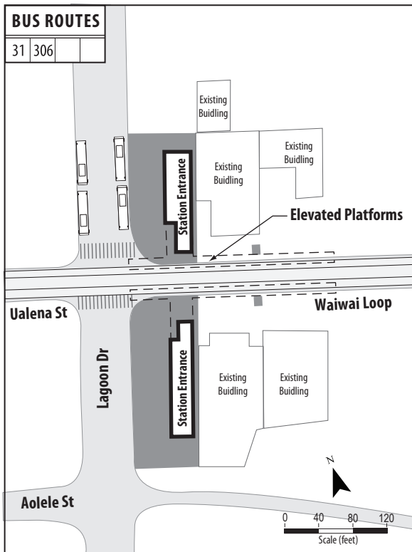
Figure 2-28 Lagoon Drive Station
