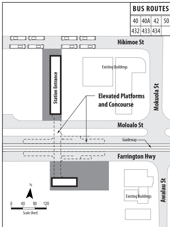
Figure 2-21 Waipahu Transit Center Station
