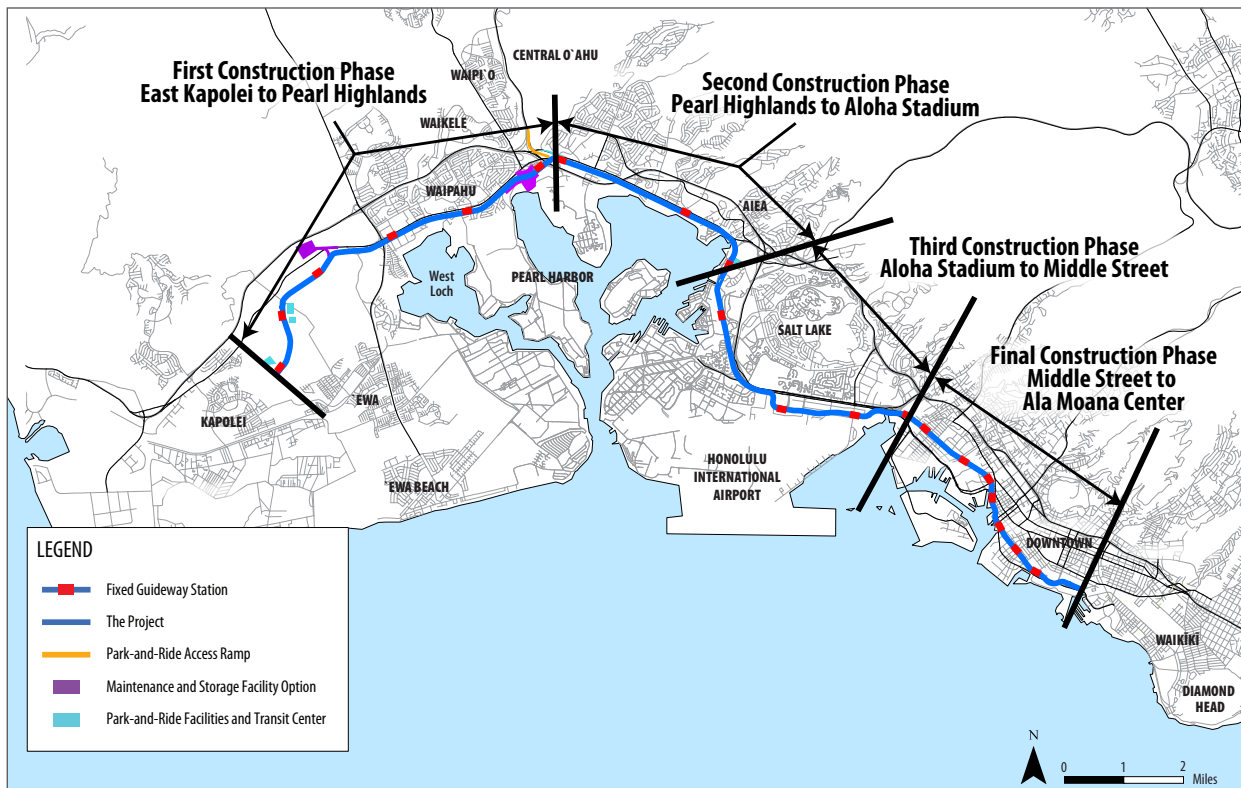
Figure 2-41 Project Construction Phases
