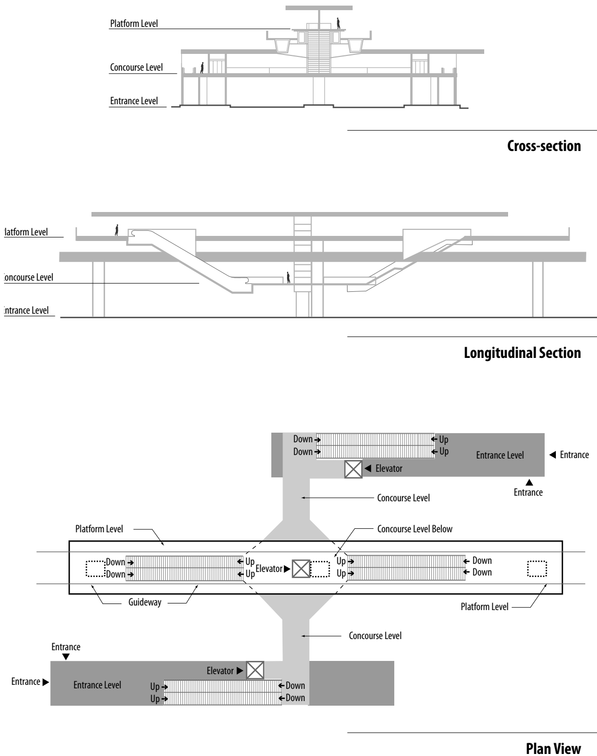
Figure 2-15 Typical Center-platform Station Configuration with a Concourse
